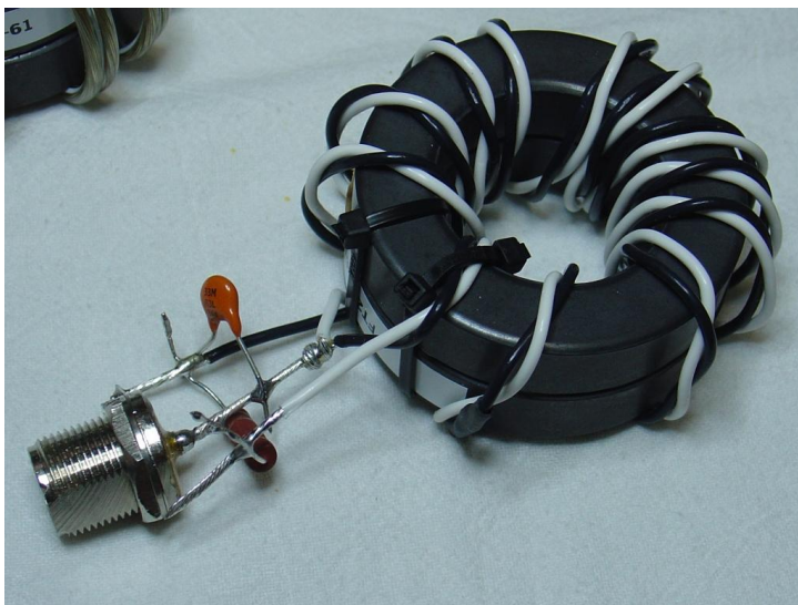
Testing: 33pf compensating capacitor and 200 ohm load
